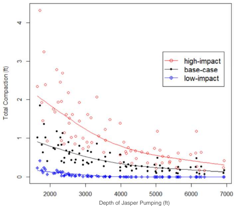
Figure 3-46. Simulated Variation of 10-year Compaction with Depth (from INTERA et al., 2018)
