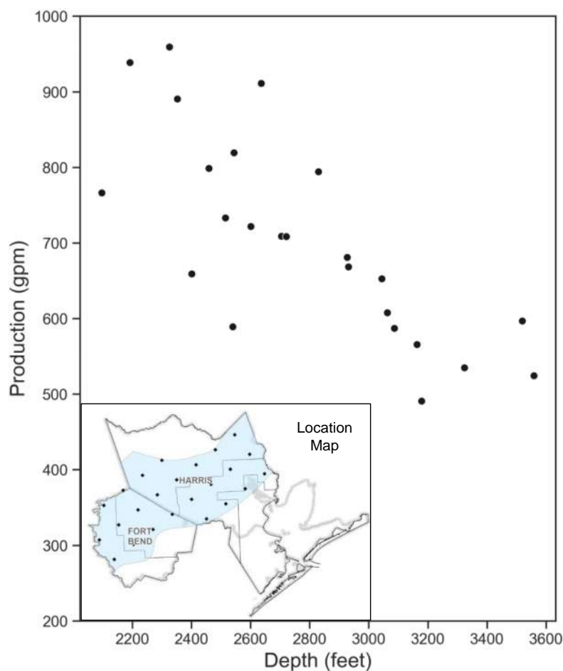
Figure 3-40. Model-Estimated Jasper Production Rate vs. Depth for 24 Brackish Well Fields Pumping Concurrently
