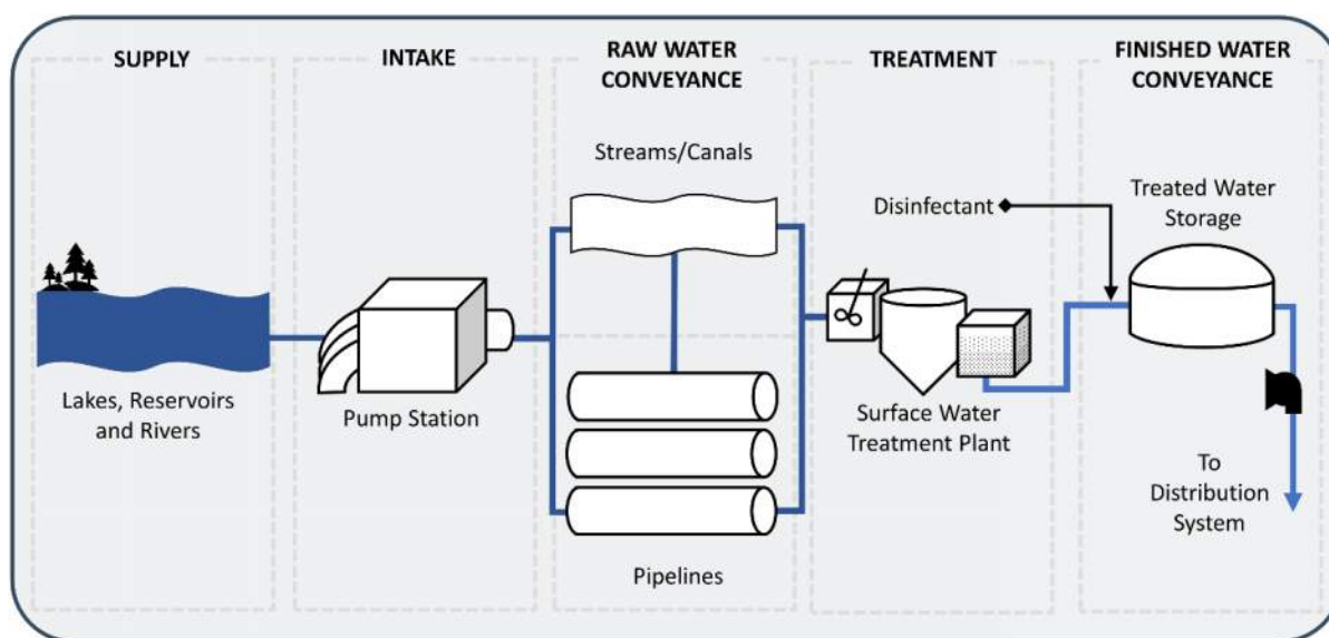
Figure 3-1. Process Flow Diagram for Surface Water Development
